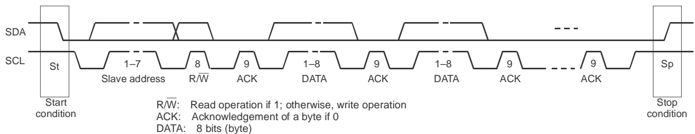
Figure 88. Packet Protocol
