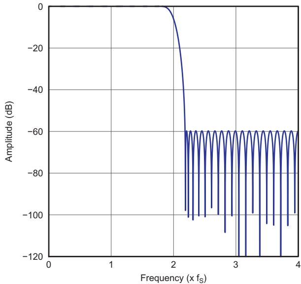
Figure 41. Normal x2 Interpolation Filter Frequency Response
