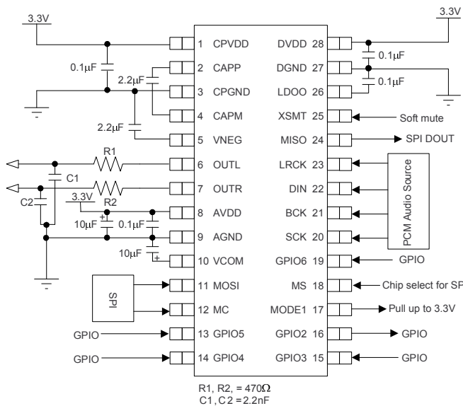
Figure 15. SPI Control, VCOM Mode, DVDD=3.3V
