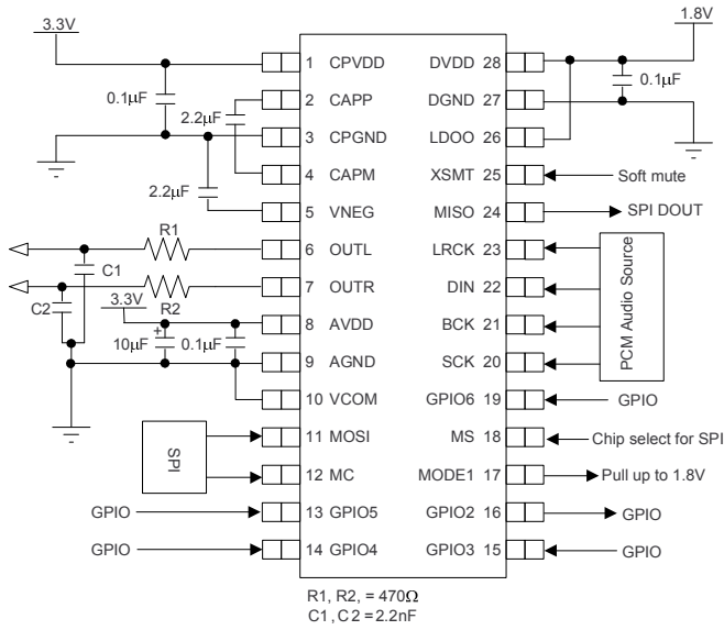
Figure 16. SPI Control, VREF Mode, DVDD=1.8V
