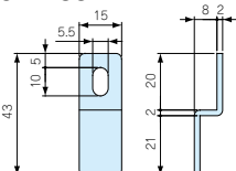
CK-35N
